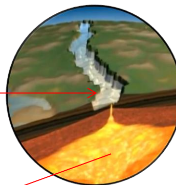
Figura 2. http://www.astromia.com/tierraluna/capastierra.htm
